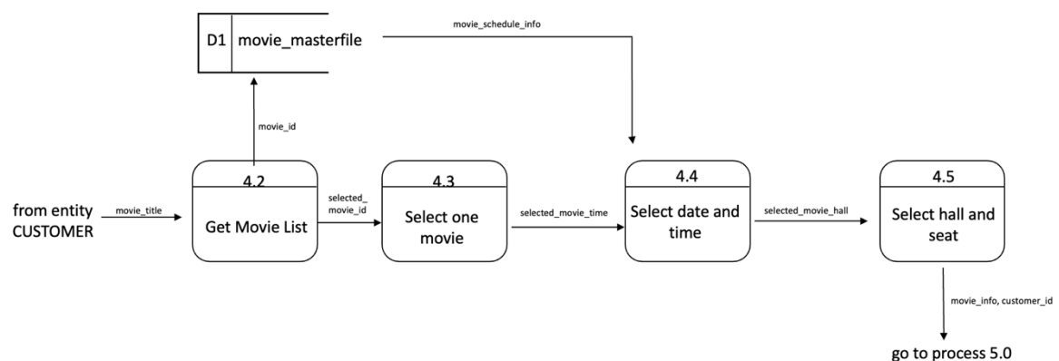
Figure 1: Logical DFD Level 1 (Process 4.0 CHOOSE MOVIE)
