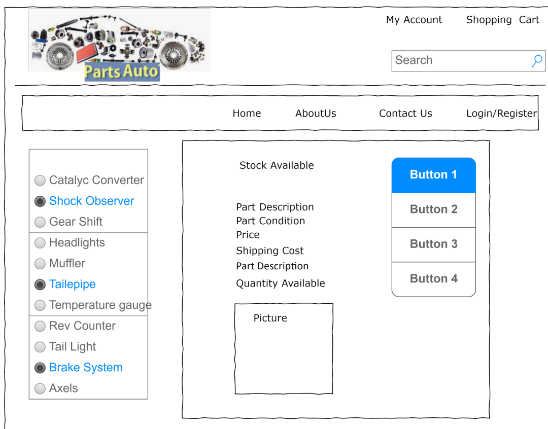
Figure 5: Initial GUI Design
